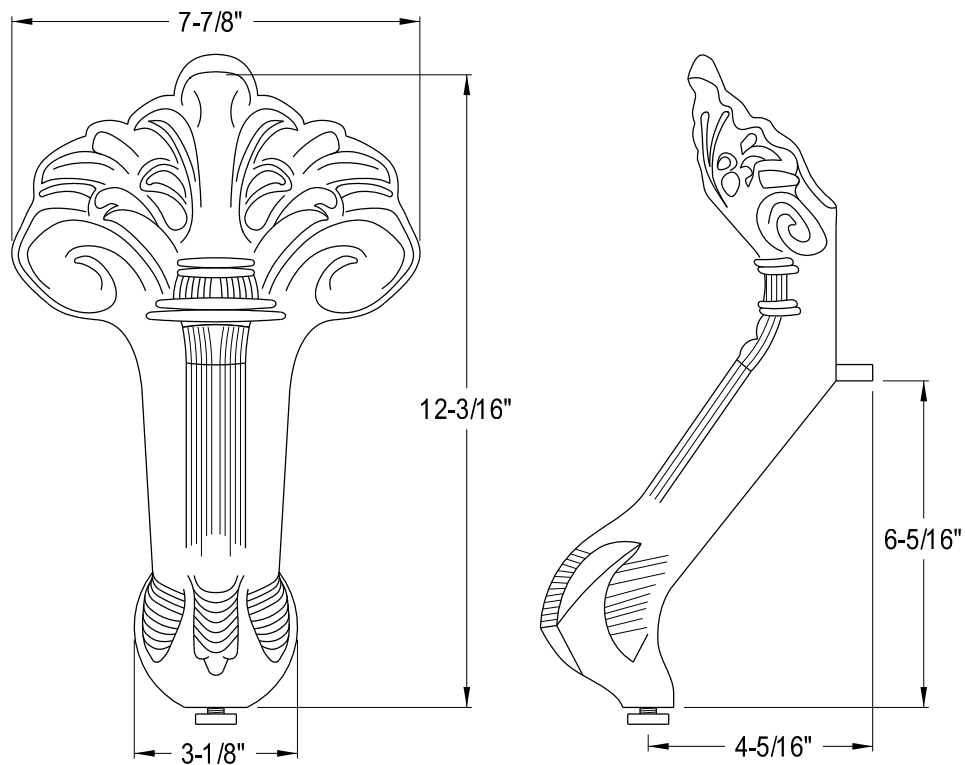
Feet with D & F marking
